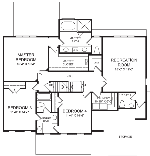
SECOND FLOOR
