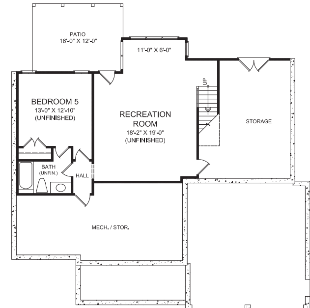
BASEMENT
